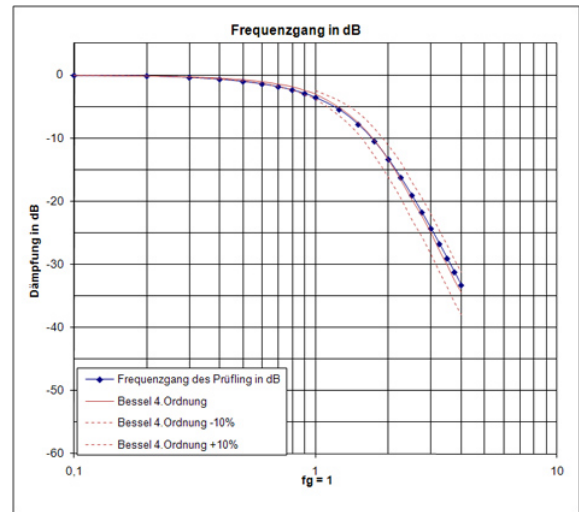
Frequency response Bessel filter
