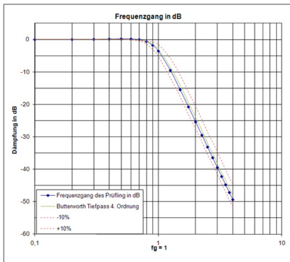
Frequency response Butterworth filter
